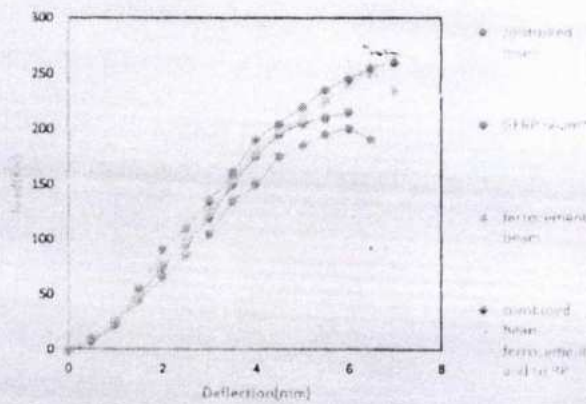
Figure 26.1 Comparison of different strengthened beams
