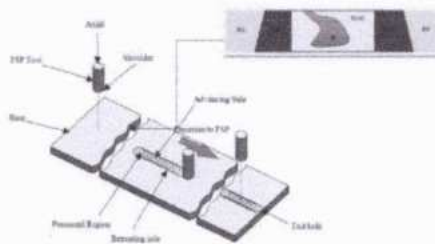
Figure 1: Schematic of Friction Stir Processing Process
