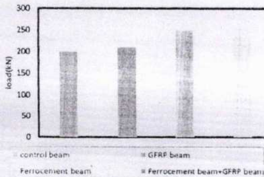
Figure 26.2 Compression of load carrying capacity of different beams
